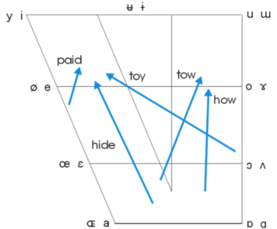
RP British English Non-Centring Diphthongs relative to the Cardinal Vowels
